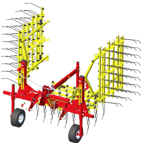
Abbildung 4: AS 450
